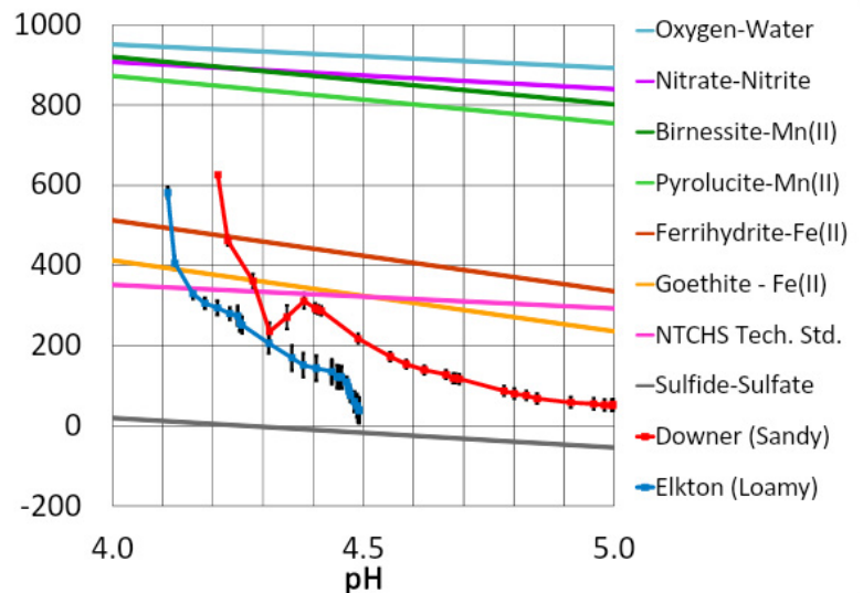
FIGURE 2. Mean Eh values (error bars show SEM) for the two sets of mesocosms relative to the ferrihydrite (Fh) stability line (0 on Y axis) and to the technical standard (TS) lines (based upon measured pH values). Both soils dropped below the Fh line within one day and they dropped below the TS line within 3 days.
