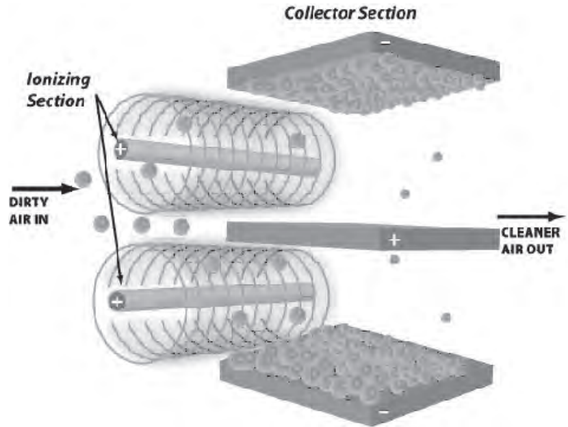
Figure 6: Two-stage electrostatic precipitator (also called an electronic air cleaner). Courtesy Honeywell
