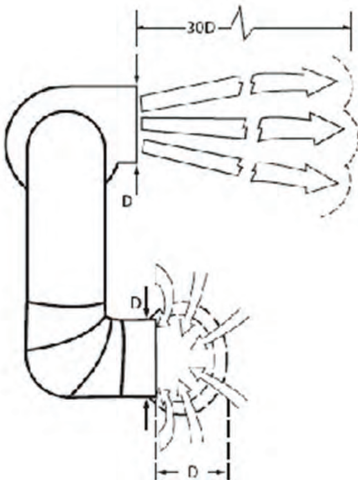
Figure 1: Standard mechanical formulas for determining effective air velocity and capture distance of air from or to a conduit.
