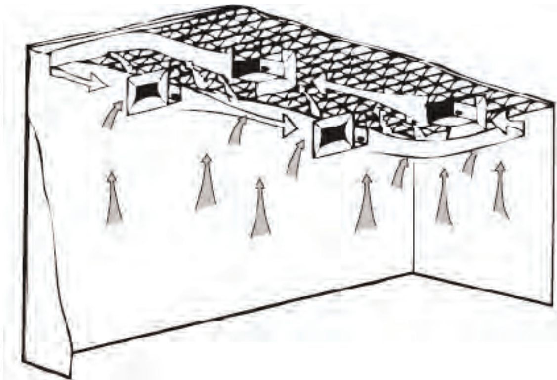
Figure 3: Description of racetrack method of general air cleaning using air cleaners suspended from the ceiling.
