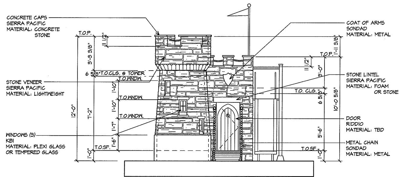
FRONT ELEV.
