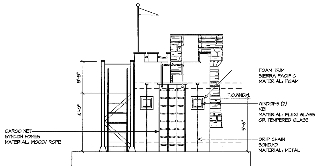
REAR ELEV.
