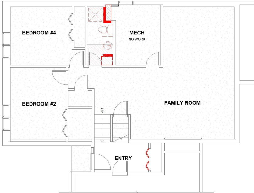
Existing Floor Plan With Demo Notations
